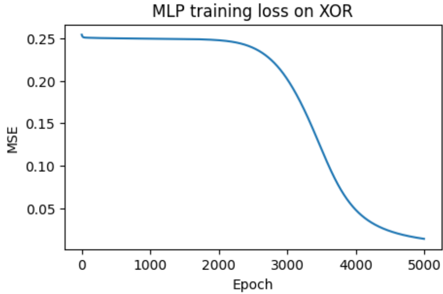
Figure 11: Training loss versus epoch for the MLP trained on the XOR gate.
