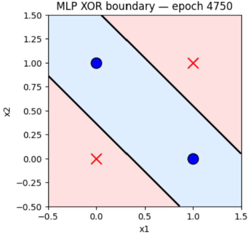
Figure 10: Final decision boundary of the MLP trained on the XOR gate.
